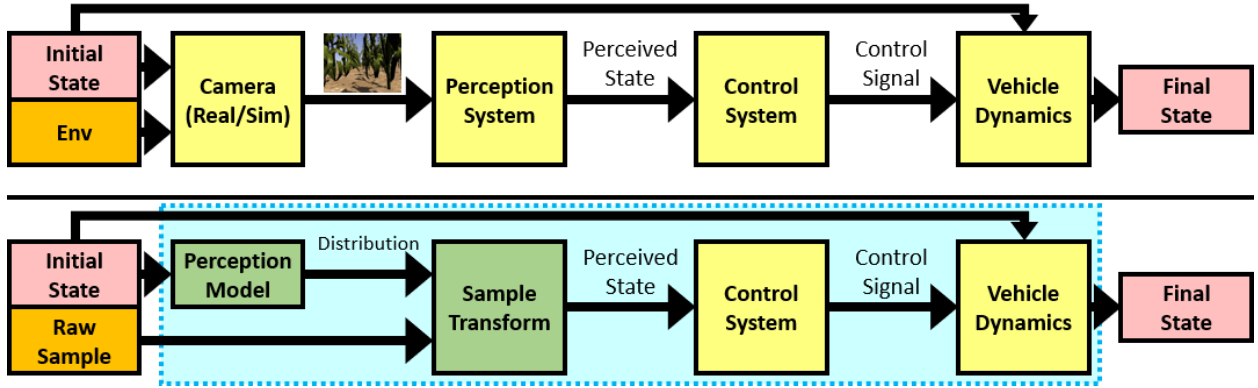
Figure 3.2: Crop-Monitor vehicle model: original (top) and abstract (bottom). GAS replaces the outlined section with a surrogate model.
