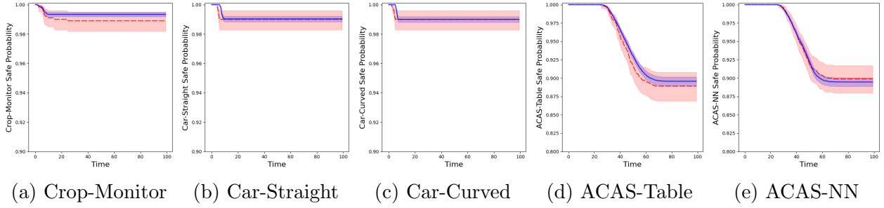
Figure 3.6: Evolution of the probability of remaining in a safe state over time. Blue solid: GAS, red dashed: MCS.
